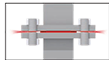
Standard scatter
